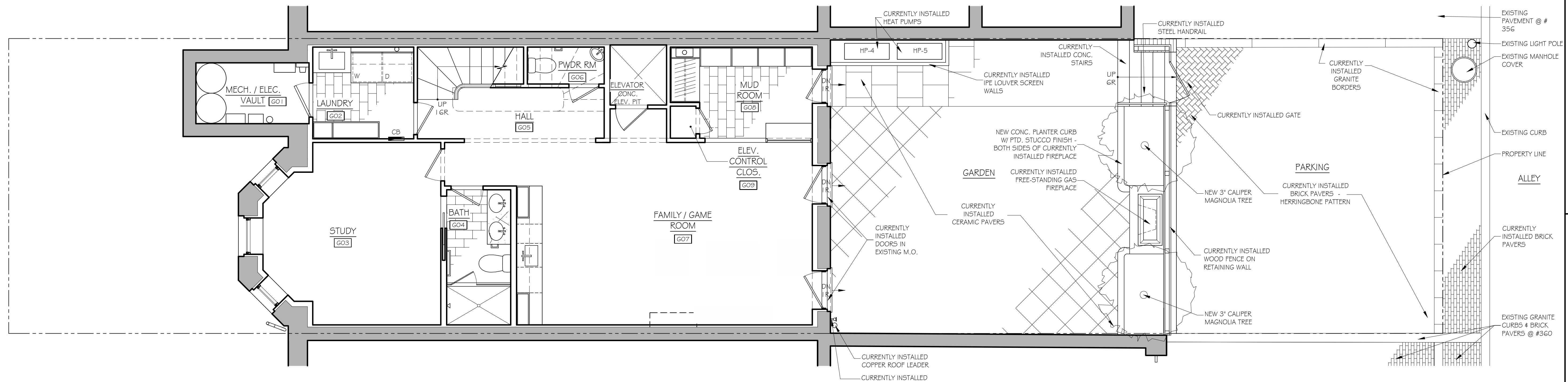
PROPOSED GARDEN FLOOR PLAN
