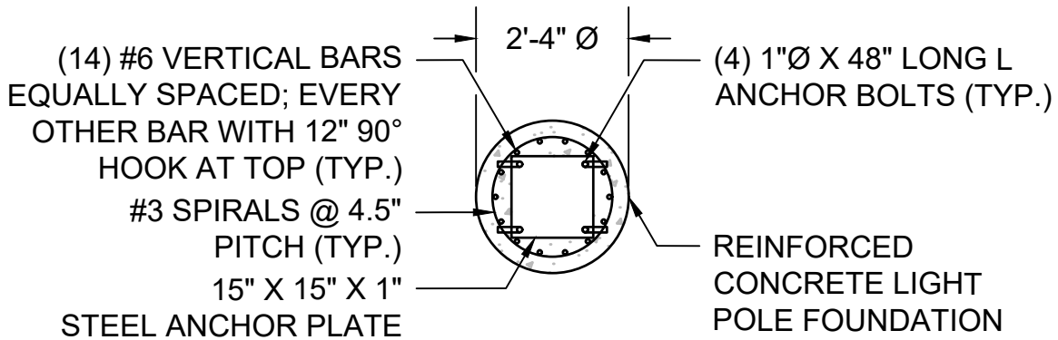
SECTION B-B
