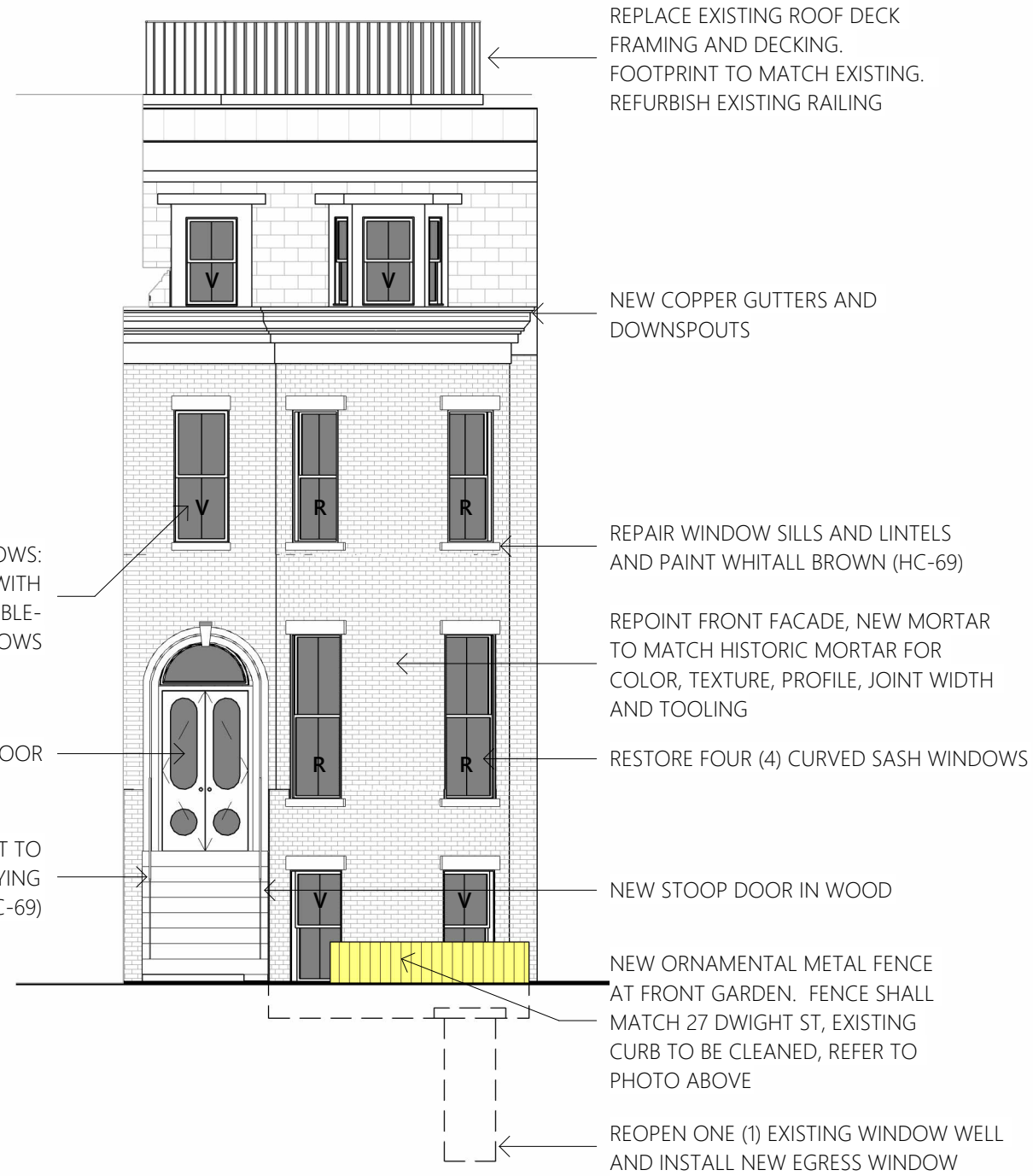
2 DWIGHT ST ELEVATION 1/8" = 1'-0"
