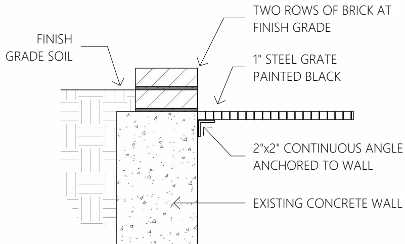
4 TOP OF WINDOW WELL 1" = 1'-0"
