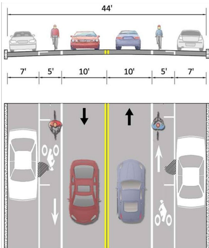
Typical bicycle lane
