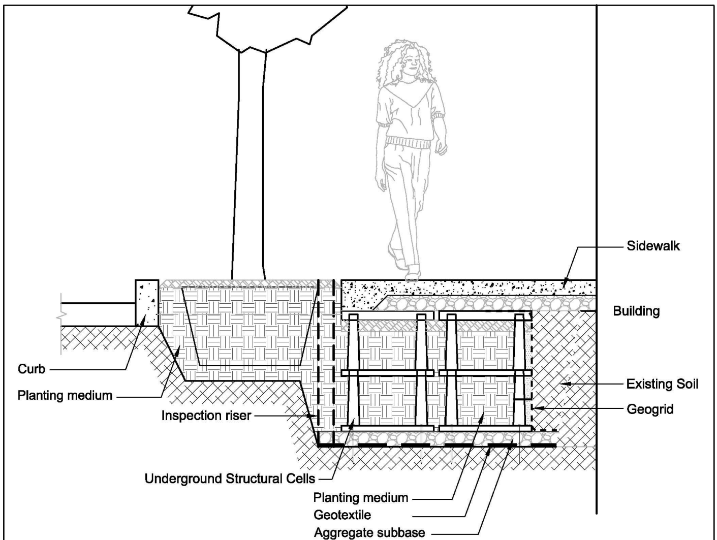
Illustration of underground structural cells for root growth beneath sidewalk.
