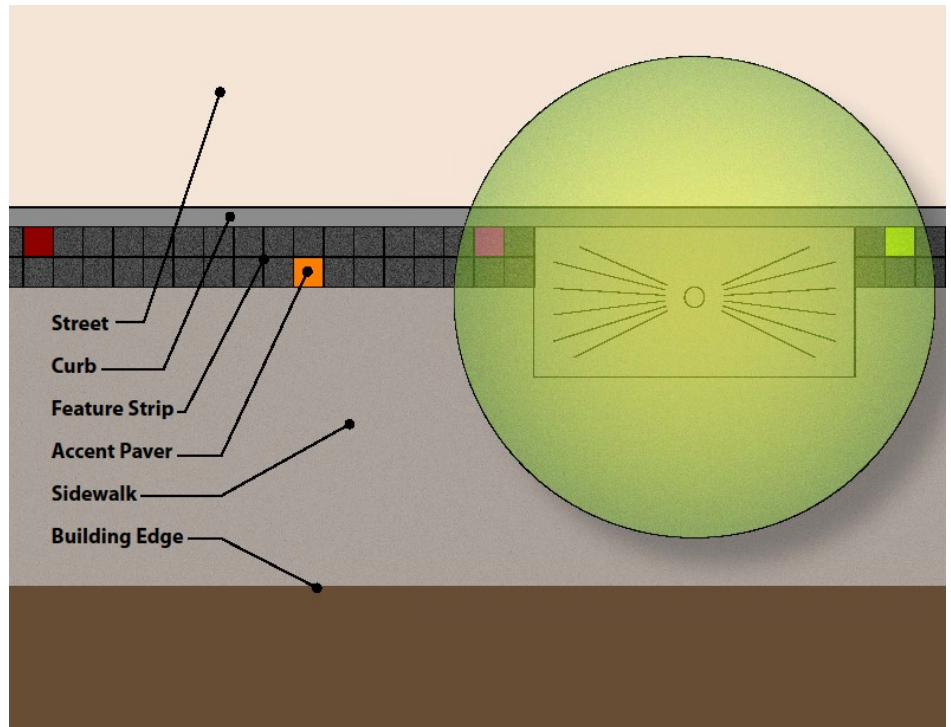
Individual pavers in the feature strip can be substituted with colored accent pavers or art pavers.
