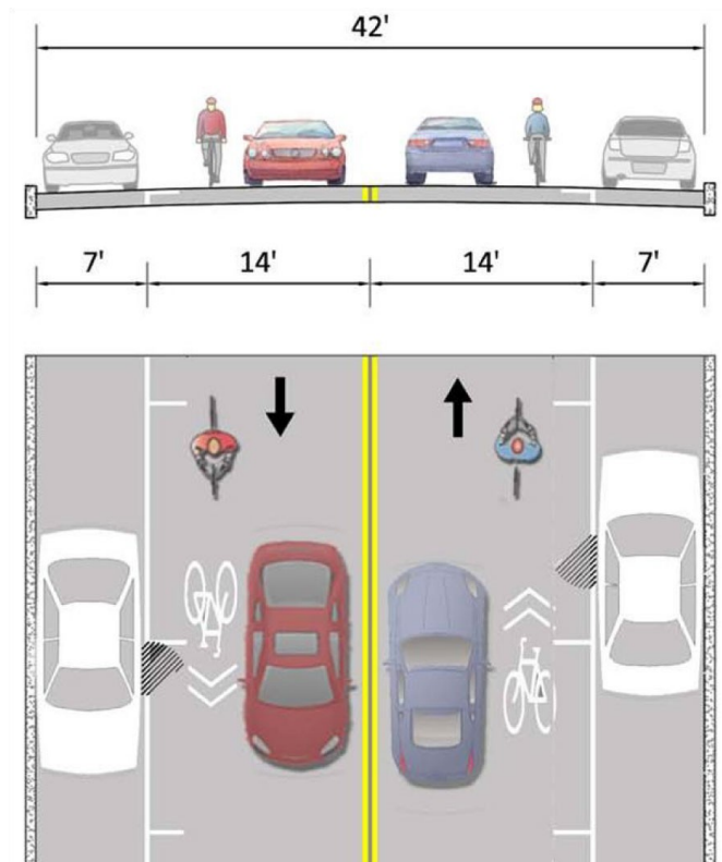
Typical shared lane
