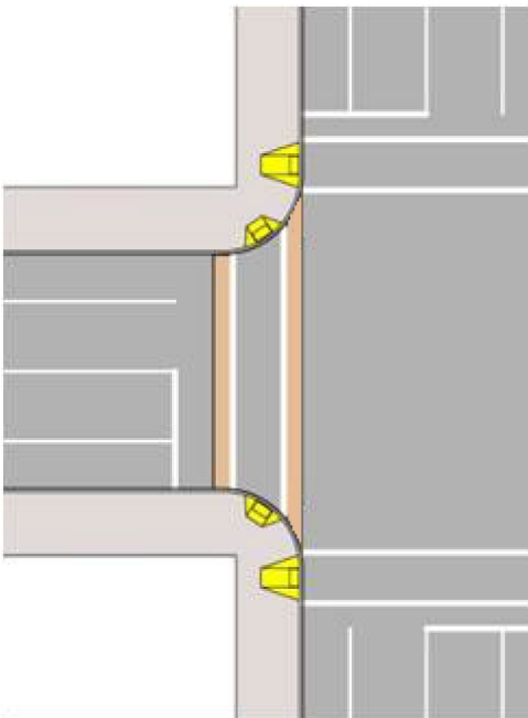
3-UP, 3-DOWN raised crosswalks are recommended across side streets.
