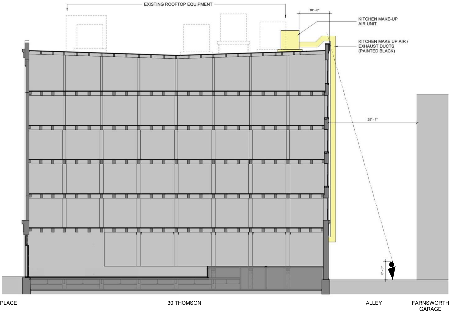
BUILDING CROSS SECTION SHOWING SIGHTLINES
