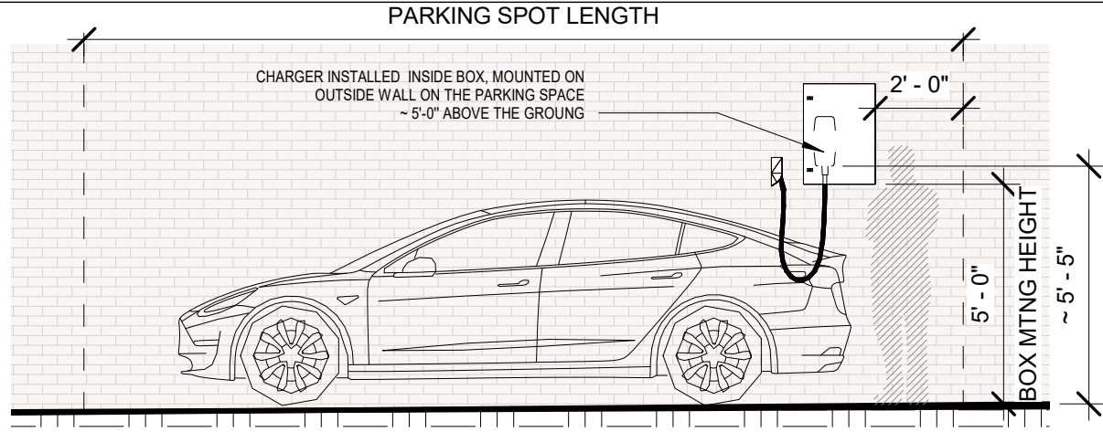
3 TESLA CHARGER ELEVATION DETAILS 1/4" = 1'-0"
