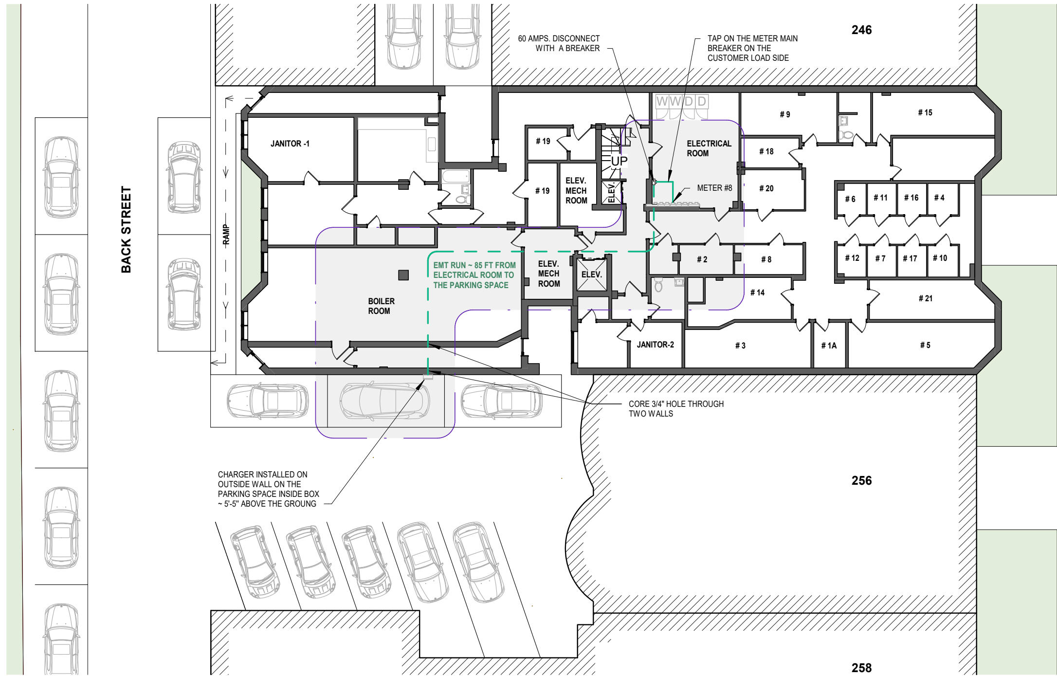
1 250 BEACON ST - PARKING PLAN 1/16" = 1'-0"
