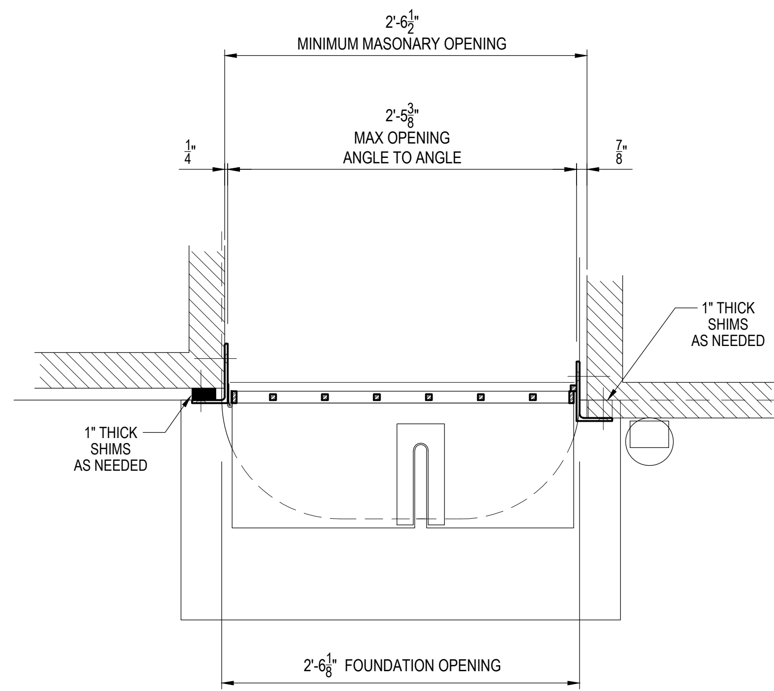
PLAN
