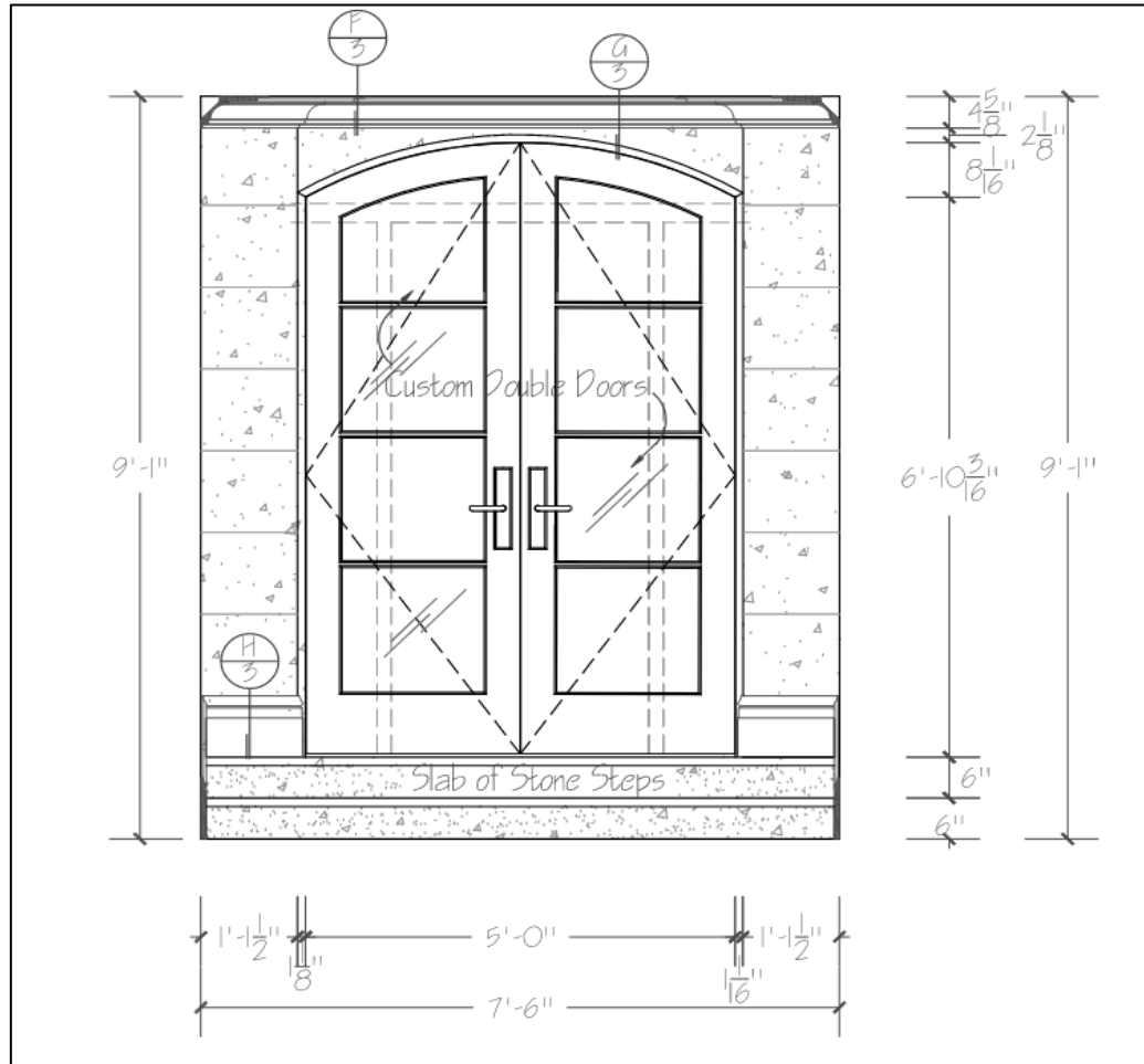
(A) Foyer Elevation Scale: 1/2" = 1'
