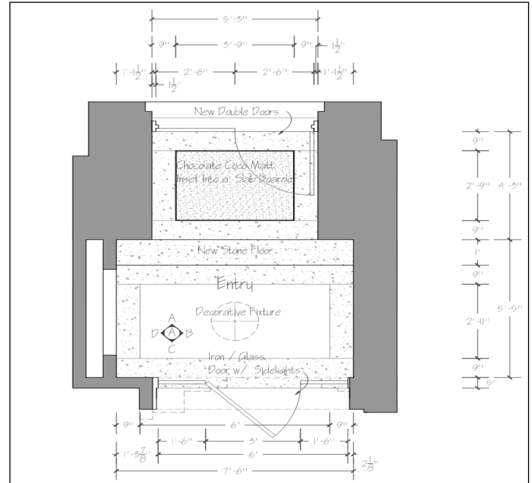
(E) Foyer Floor Plan Scale: 1/2" = 1'
