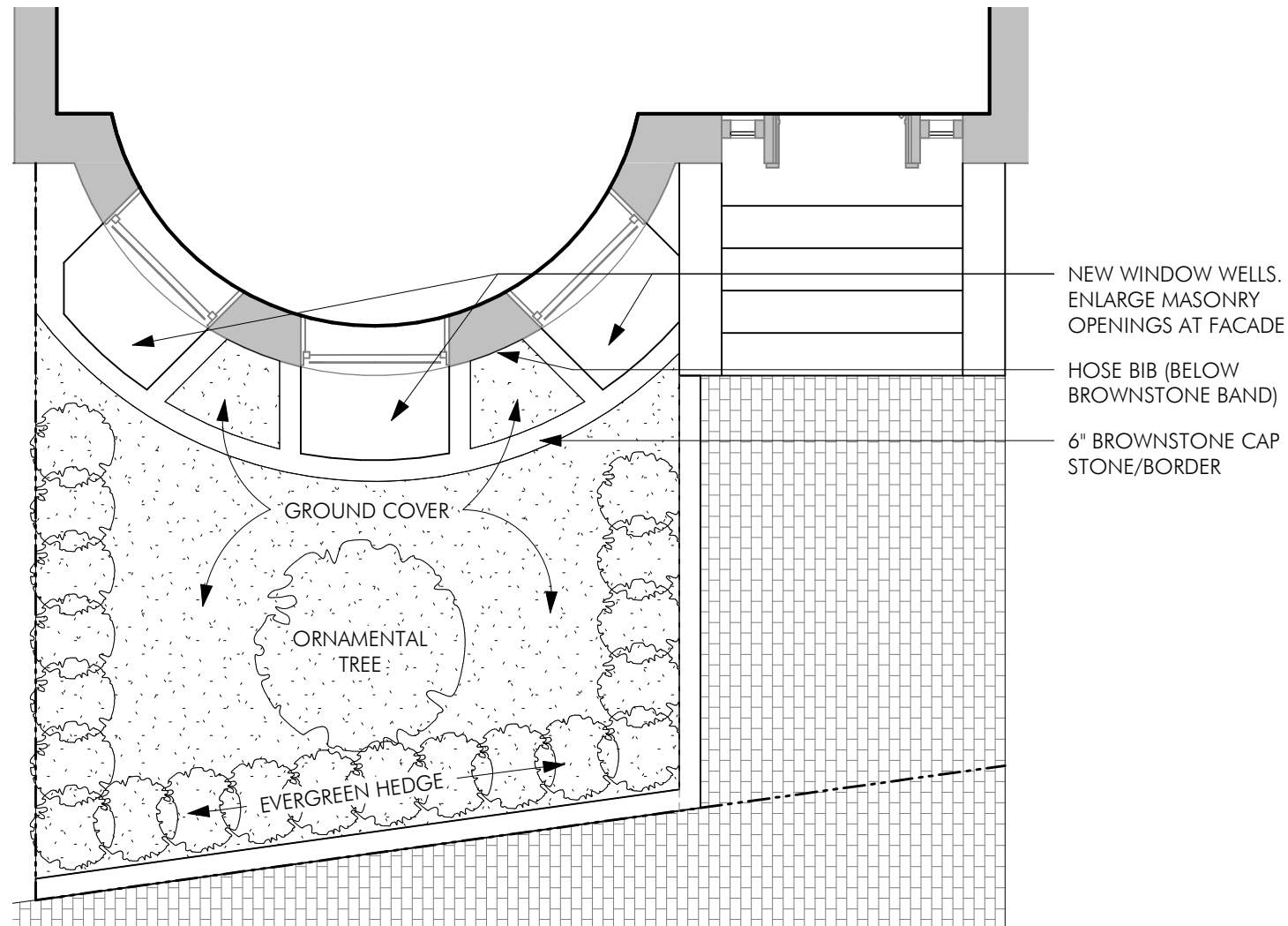
1 PROPOSED FRONT YARD PLAN 1/4" = 1'-0"
