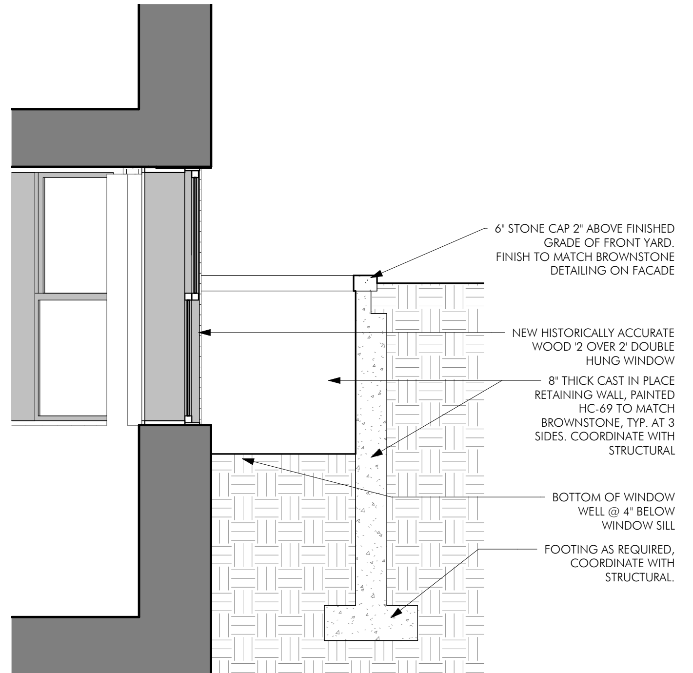
2 WINDOW WELL SECTION 1/2" = 1'-0"
