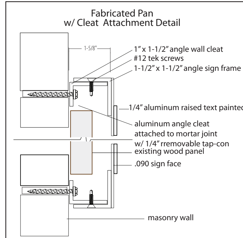
A Section - Wall Sign Attachment 1:10 scale
