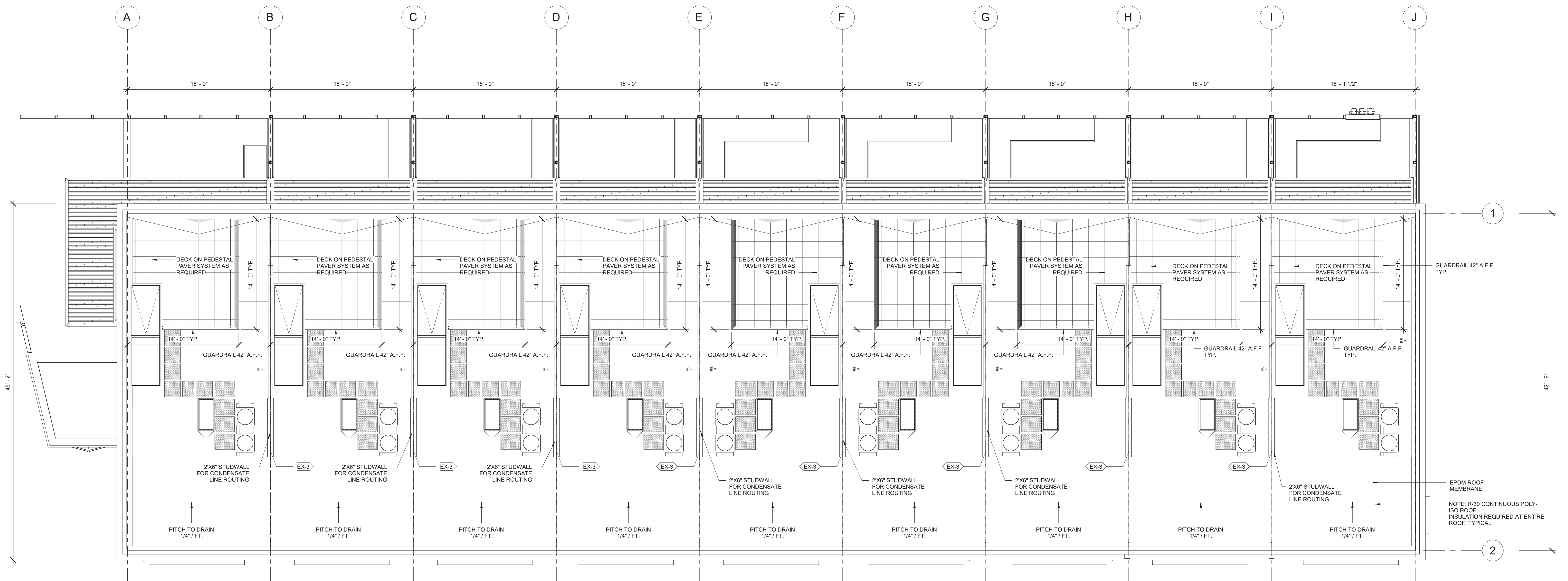
3 ROOF PLAN @ ROOF DECK 3/16" = 1'-0"
