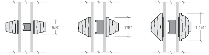
Putty Glaze and Ogee Grilles Wood Exterior - Wood Interior 1
