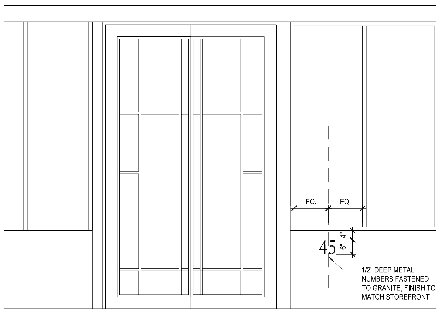
2 ADDRESS SIGN: 6" HIGH OPTION SCALE: 1/2" = 1'-0"
