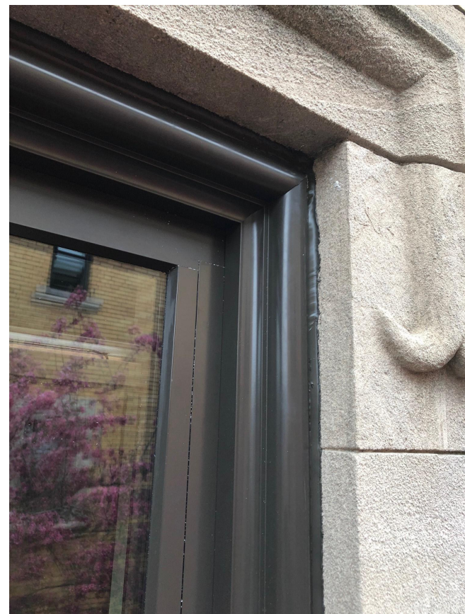
DETAIL F - PROPOSED WINDOW BRICK MOLD AT JAMB / HEAD
