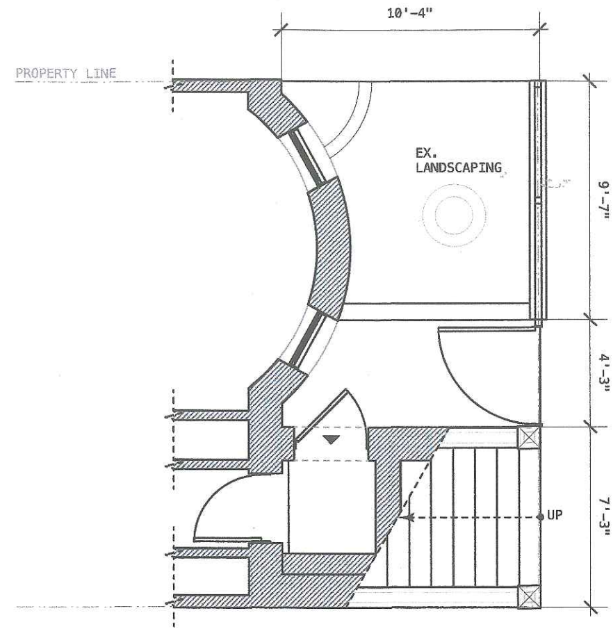
20 EXISTING 1ST FLOOR - FRONT YARD SCALE: 3/16" = 1'-0"
